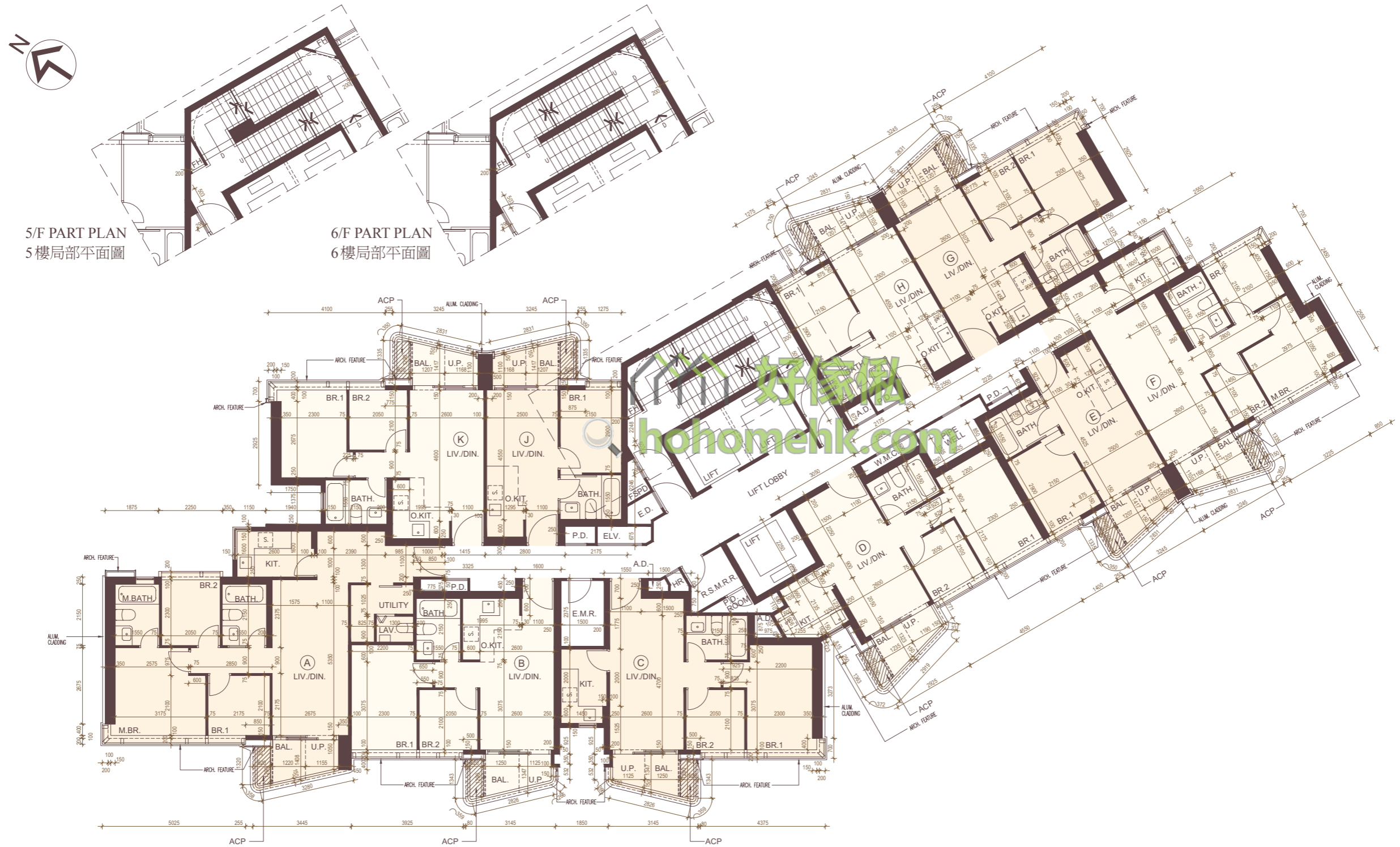
5/F - 12/F and 15/F - 20/F FLOOR PLAN 5樓至12樓及15樓至20樓平面圖
