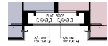
PART PLAN OF 3/F 3樓部分平面圖
