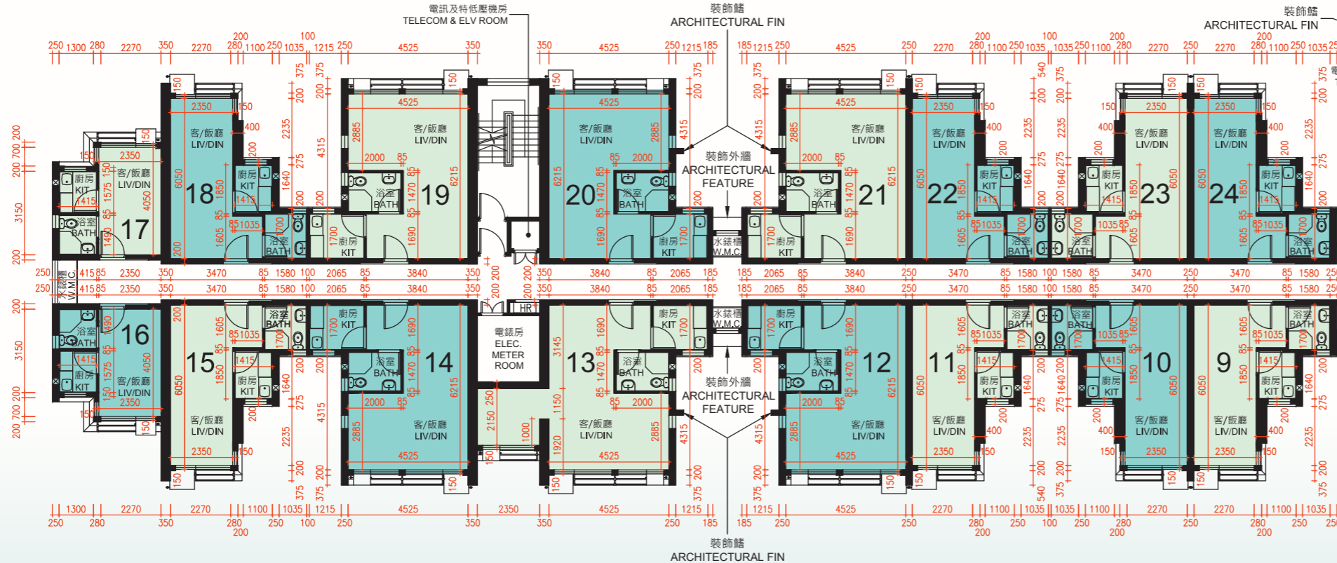
3樓部分平面圖 PART PLAN AT 3/F
